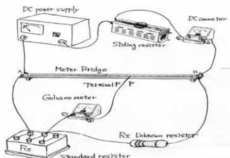
Figure 1 Experimental Equipment
